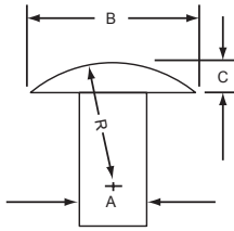
STANDARD BRAZIER HEAD ALUMINUM RIVETS
